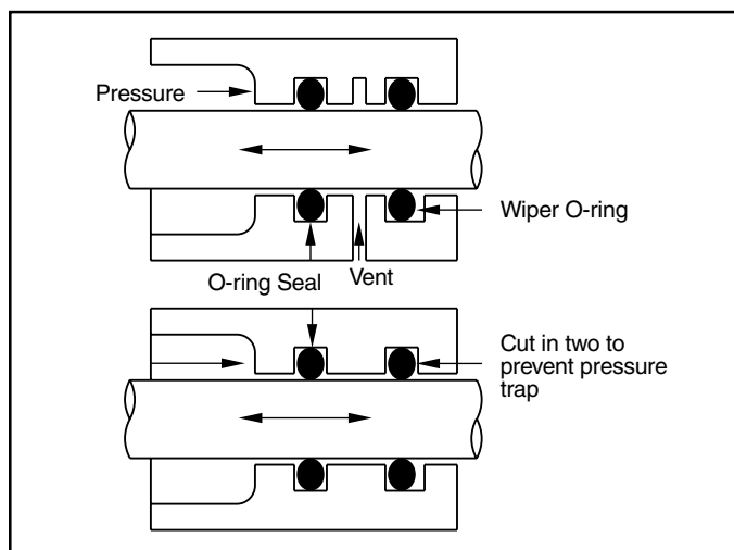
Figure 1-14: Wiper Installation
