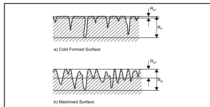
Figure 5-6: Surfaces Produced by Roller Burnishing (a) and by Normal Machining (b)
