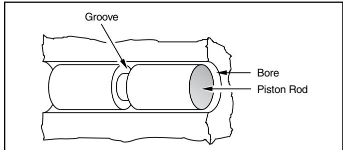
Figure 1-2: Basic Gland
