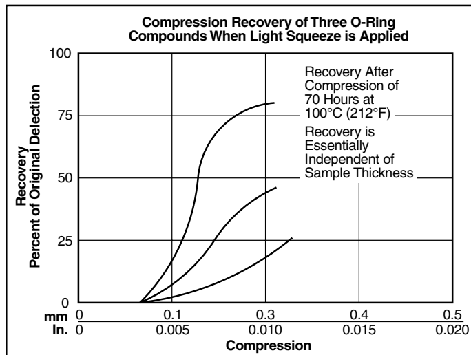
Figure 3-5: Compression Recovery of Three O-ring Compounds When Light Squeeze is Applied
