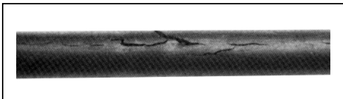
Figure 10-5: O-Ring Damaged by Explosive Decompression
