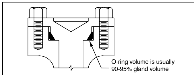
Figure 1-13: Crush Installation
