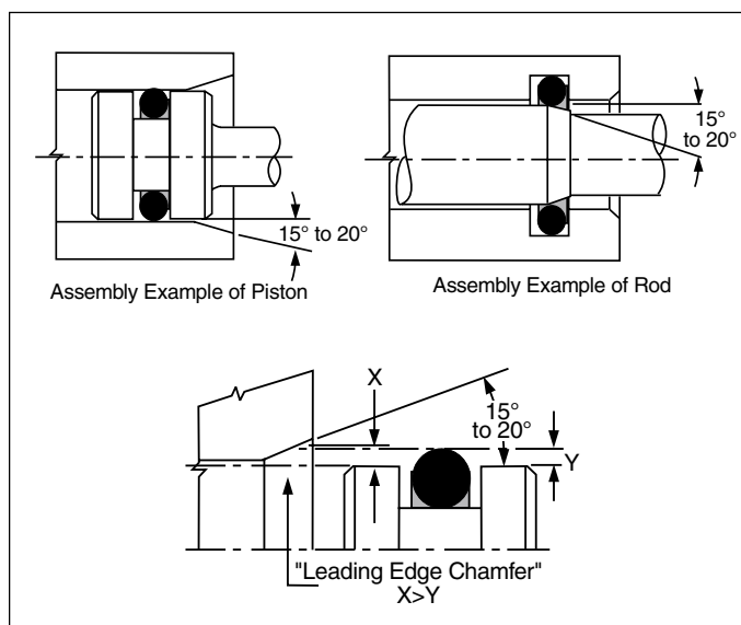
Figure 10-7: Chamfers
