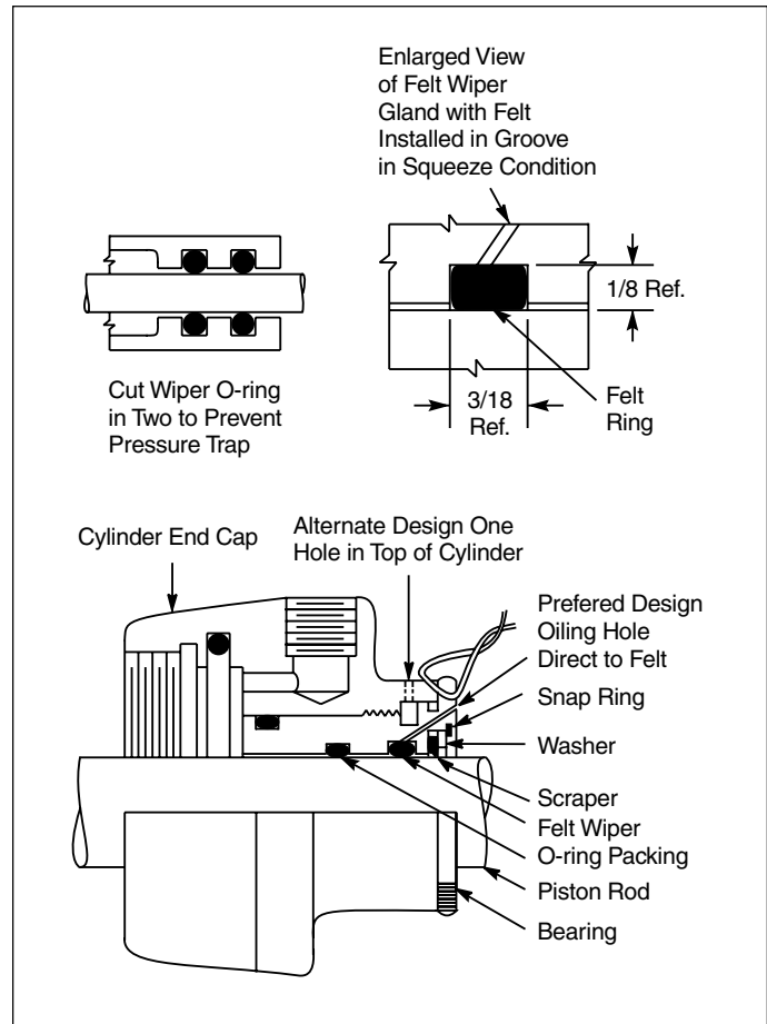
Figure 5-2: Lubrication Between Scraper and Seal Rings
