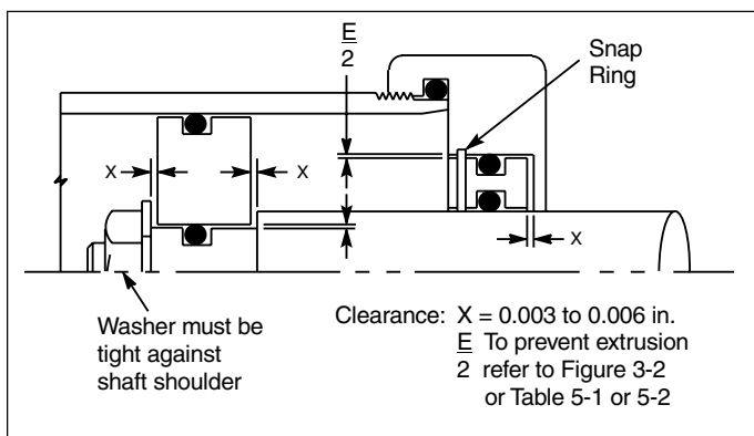
Figure 5-18: Floating Gland
