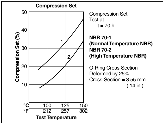
Figure 2-12: Compression Set vs. NBR 70 Compounds
